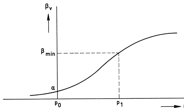
Fig. 3. The power of the test by variables.
